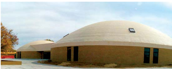
TEXHOMA PUBLIC SCHOOLS (Texhoma, Ok) 2000 108' Diameter by 22.5 High Classrooms and Gymnasium - 2 Domes
